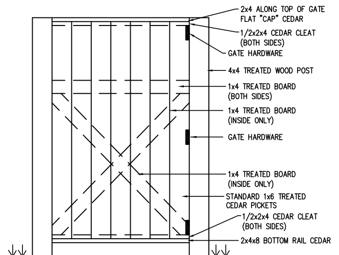
GATE FOR PRIVACY FENCE DETAIL
