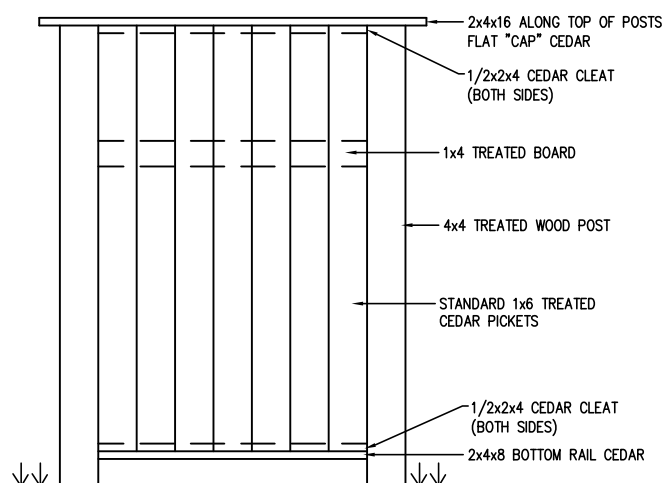
6' WOOD PRIVACY FENCE w/ CAP DETAIL
