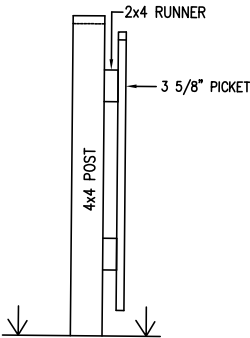
SIDE VIEW OF PICKET FENCE
