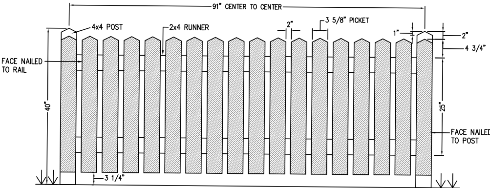
FRONT VIEW OF PICKET FENCE
