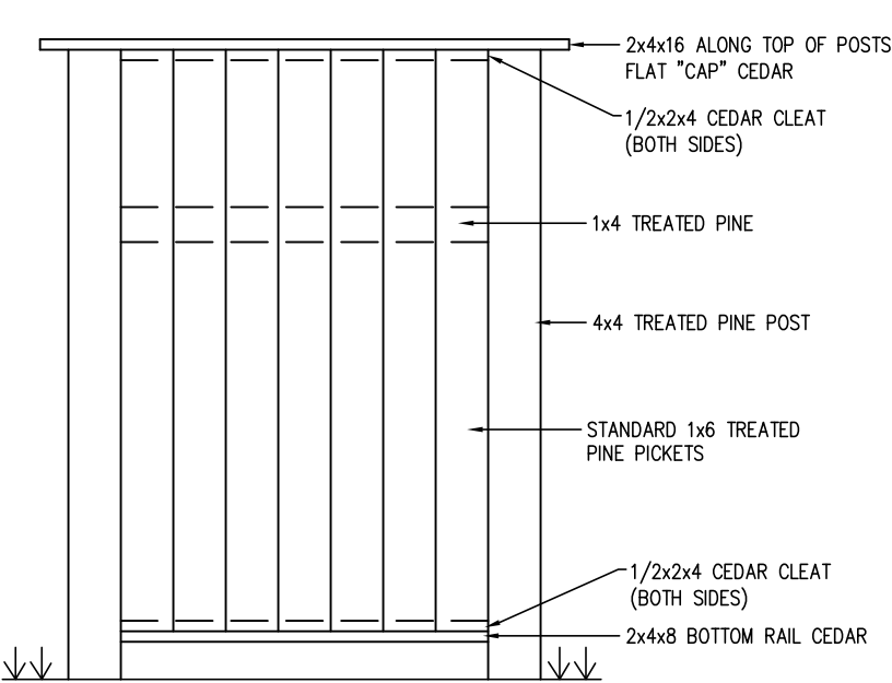
6' WOOD PRIVACY FENCE DETAIL
