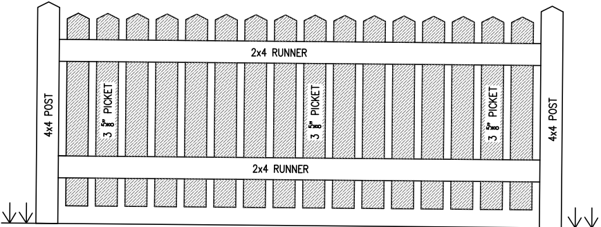
REAR VIEW OF PICKET FENCE
