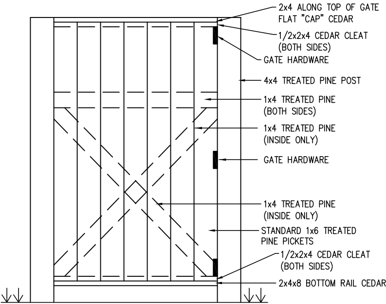
GATE FOR PRIVACY FENCE DETAIL
