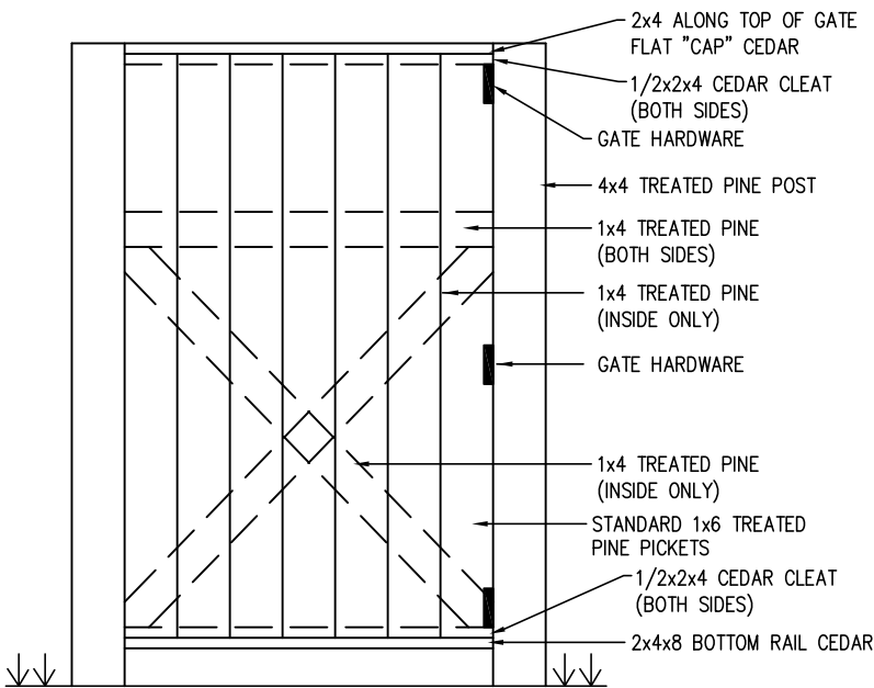
GATE FOR PRIVACY FENCE DETAIL
