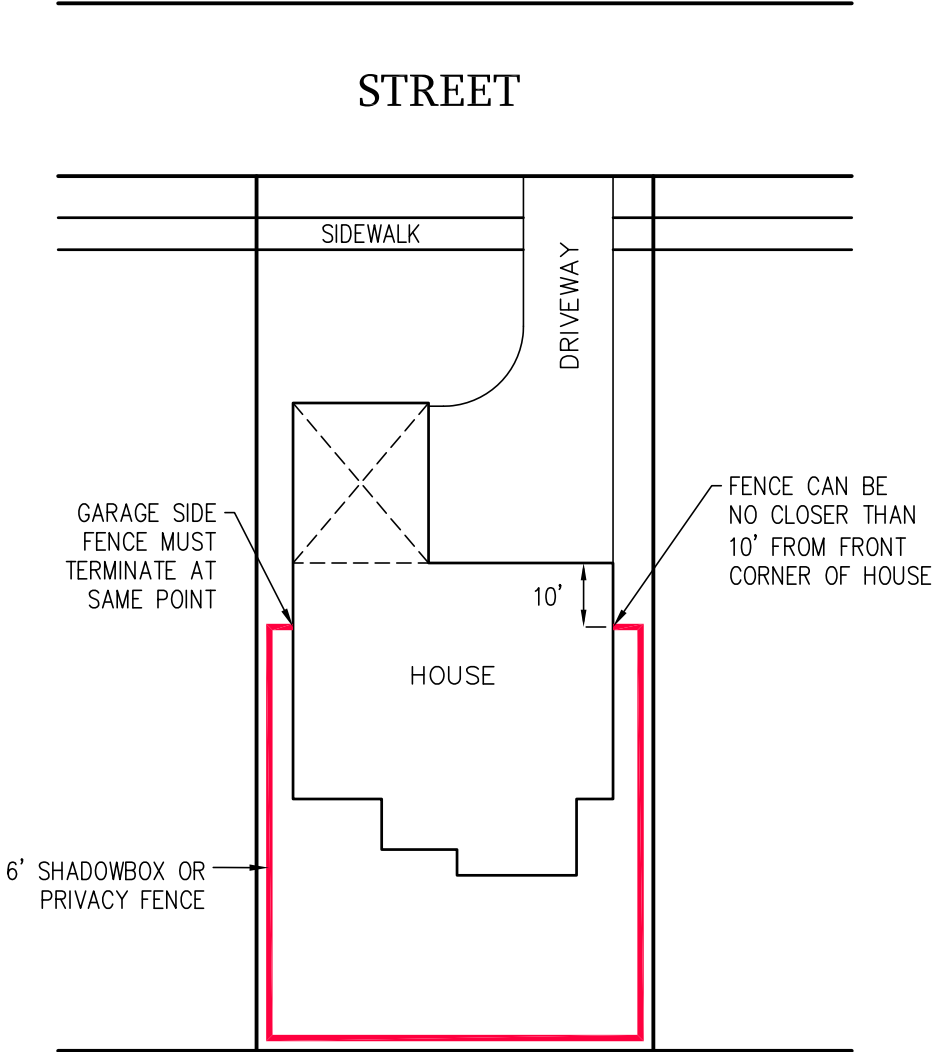
PLAN VIEW OF FRONT LOAD LOT (TYPICAL)
