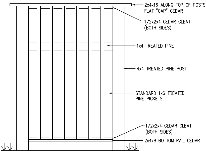
6' WOOD PRIVACY FENCE DETAIL
